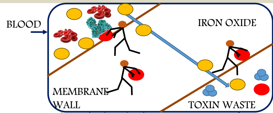
The mechanism of toxin transport across membrane
